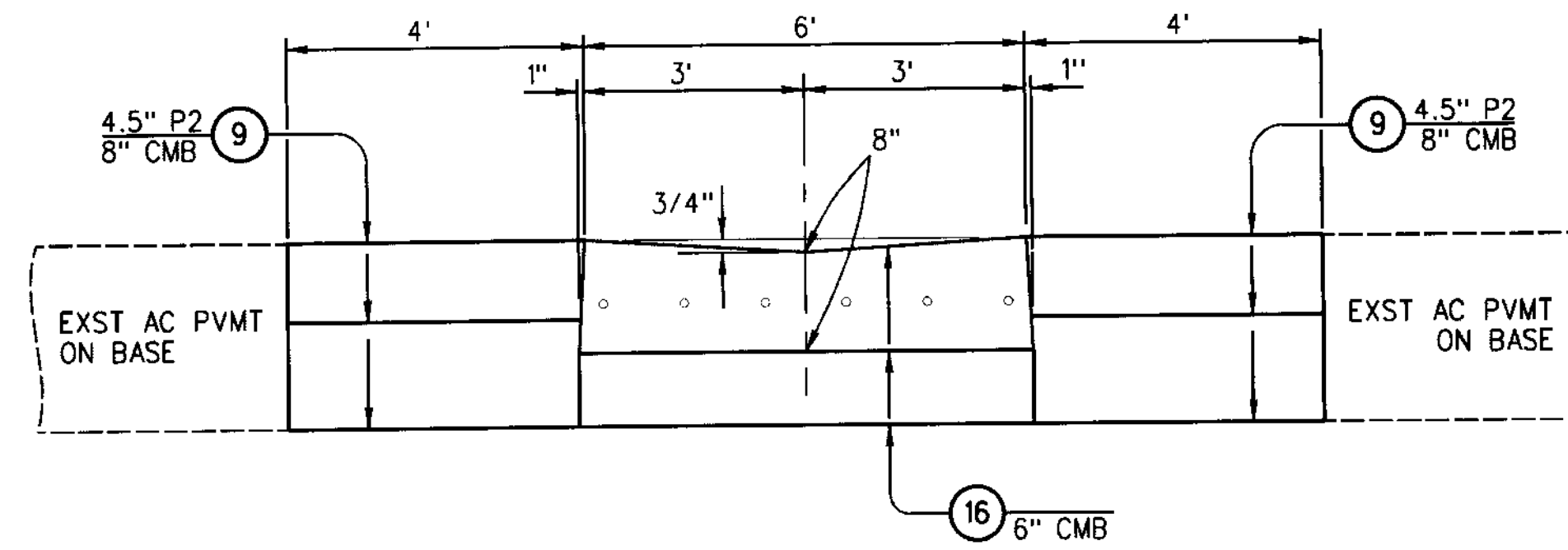
SECTION F-F NO SCALE
